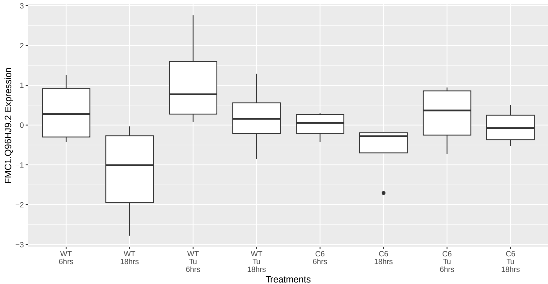
FMC1.Q96HJ9.2 occurs in the midnightblue module
