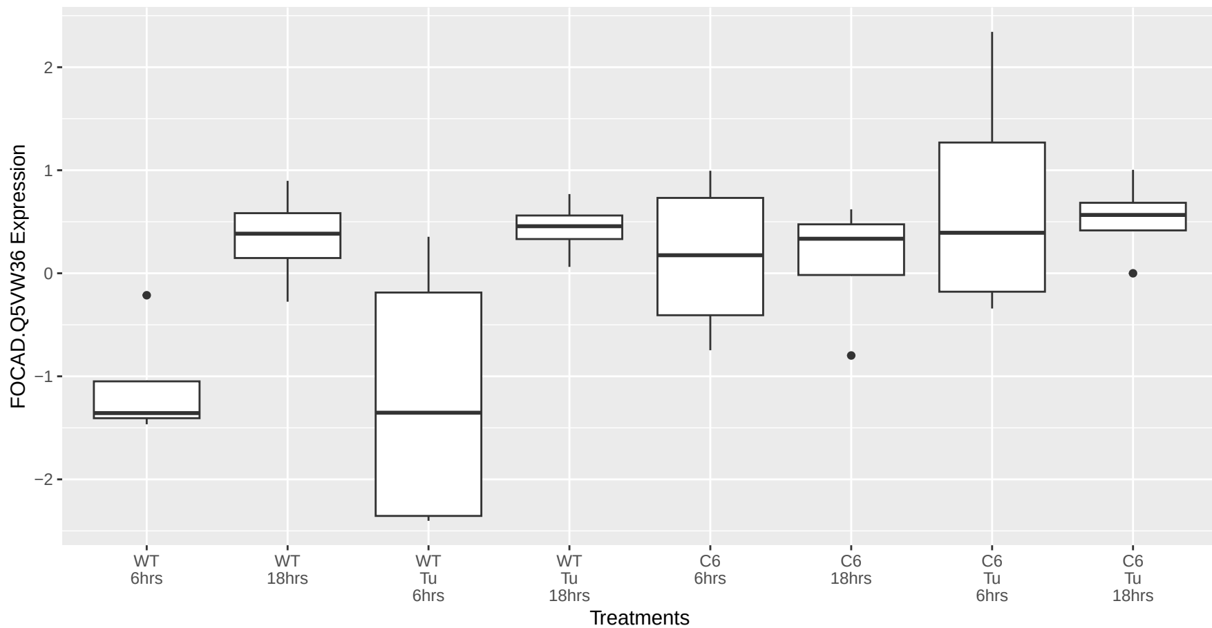
FOCAD.Q5VW36 occurs in the magenta module
