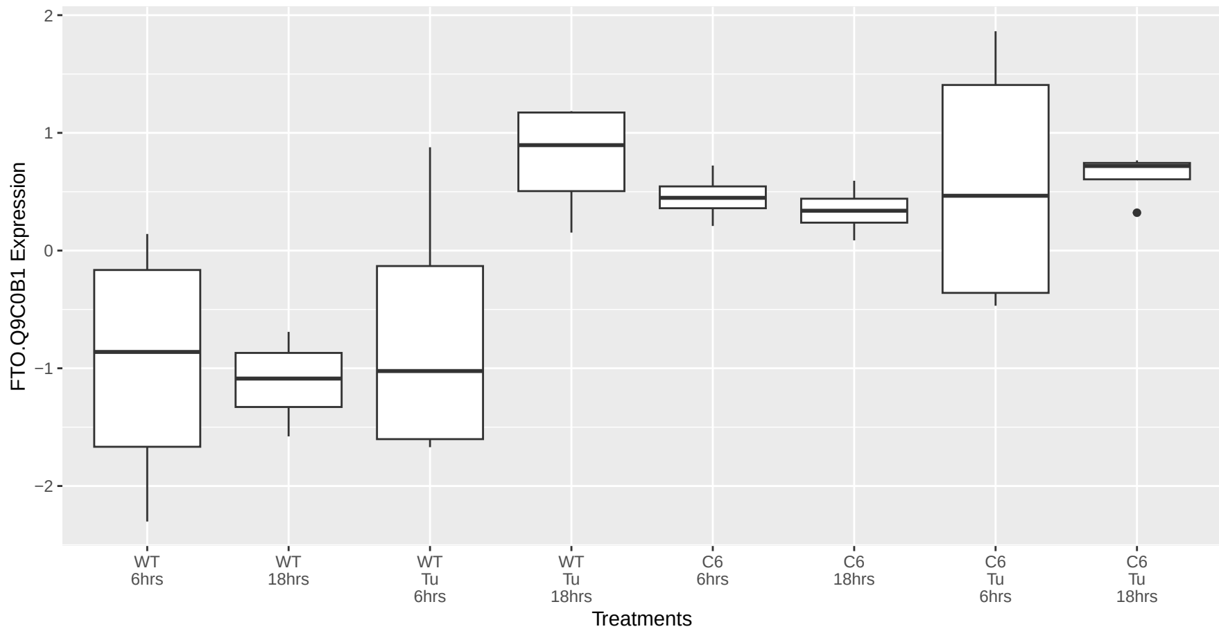
FTO.Q9C0B1 occurs in the black module
