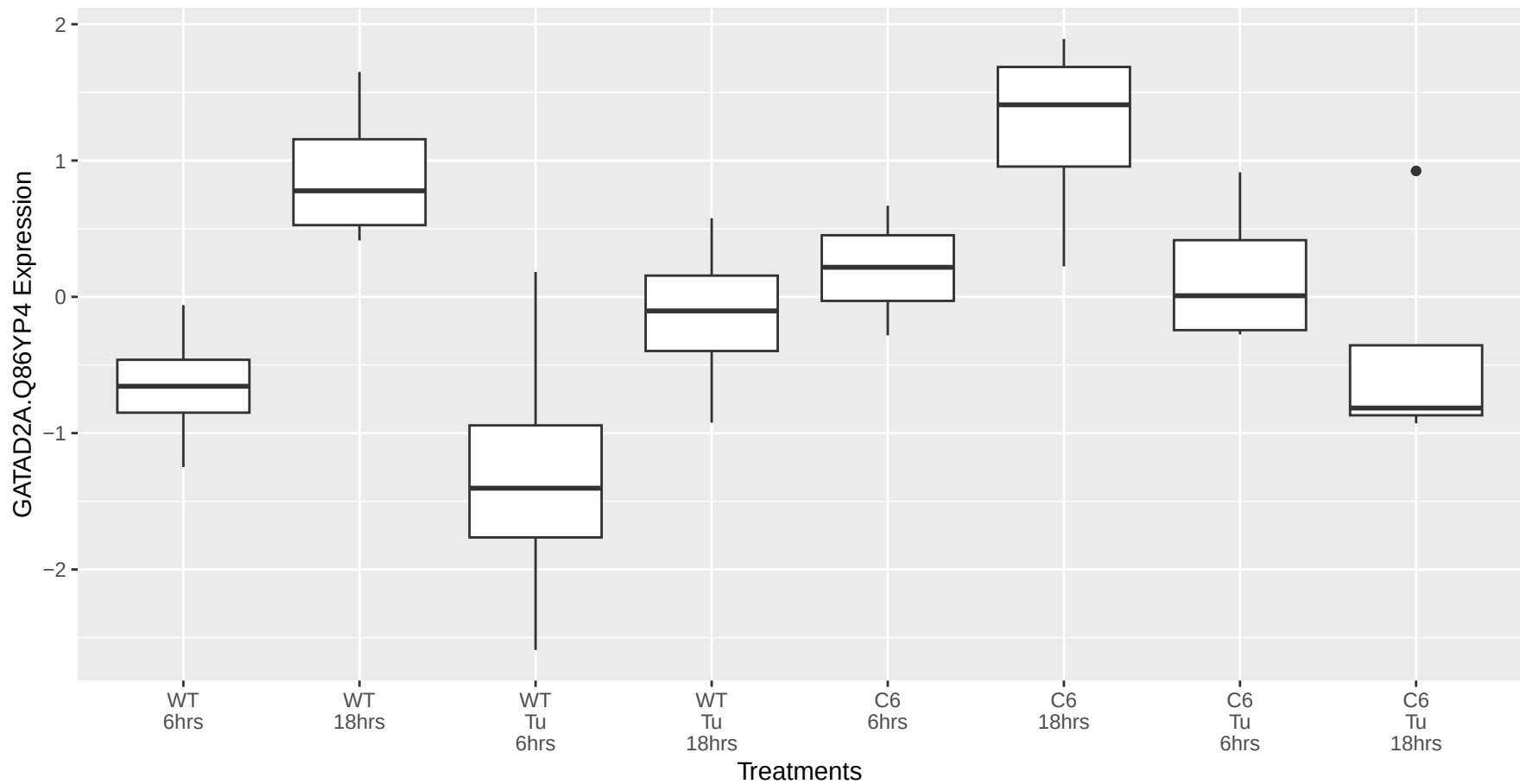
GATAD2A.Q86YP4 occurs in the greenyellow module
