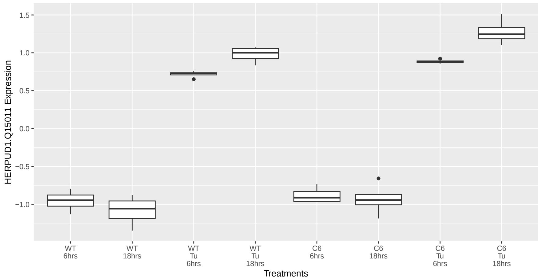
HERPUD1.Q15011 occurs in the pink module
