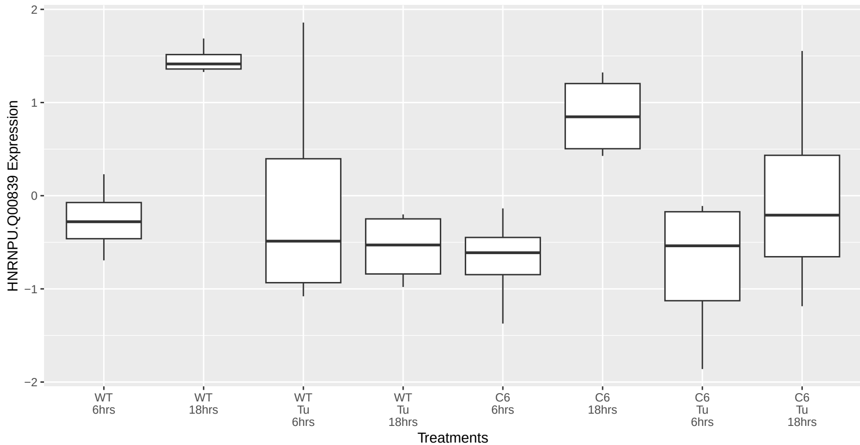
HNRNPU.Q00839 occurs in the midnightblue module
