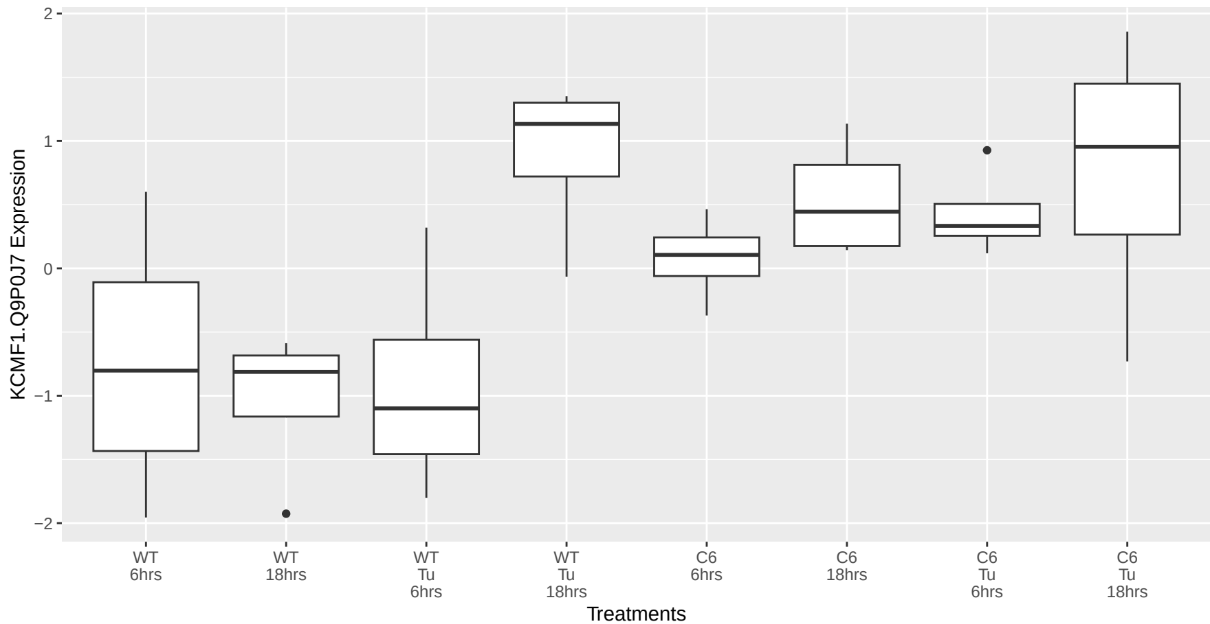
KCMF1.Q9P0J7 occurs in the blue module
