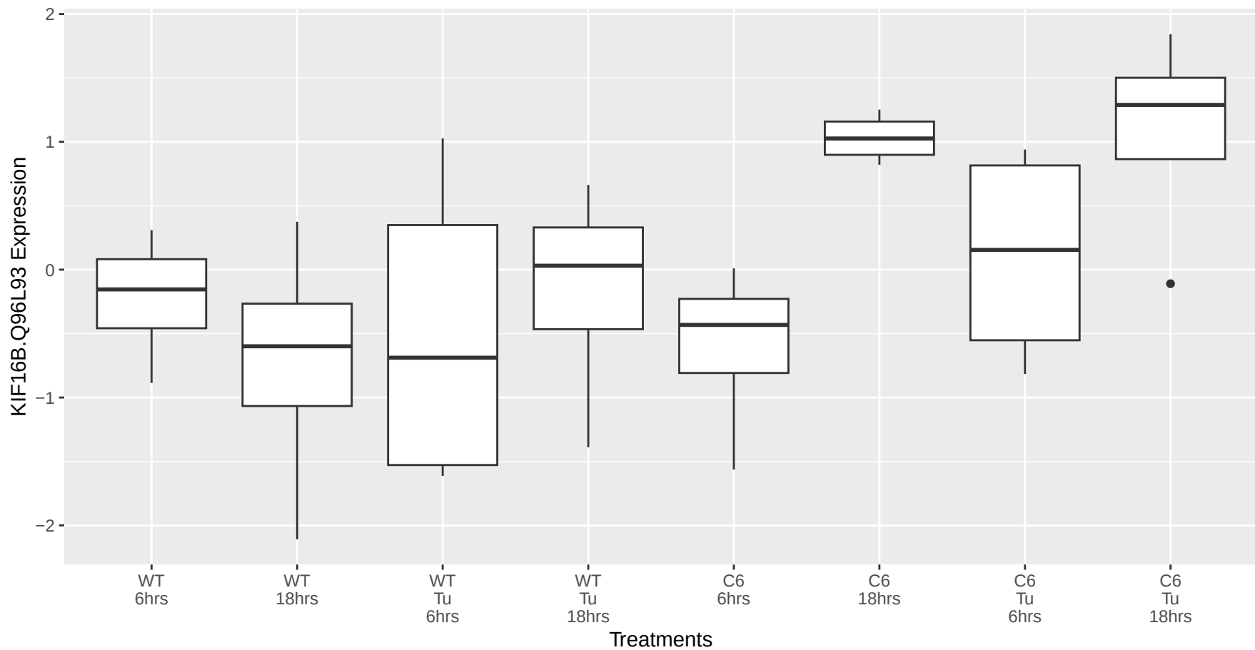
KIF16B.Q96L93 occurs in the black module
