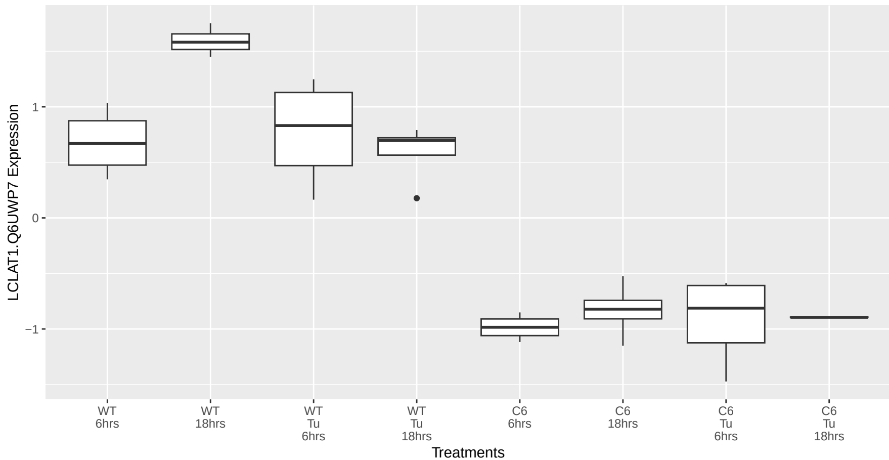
LCLAT1.Q6UWP7 occurs in the brown module
