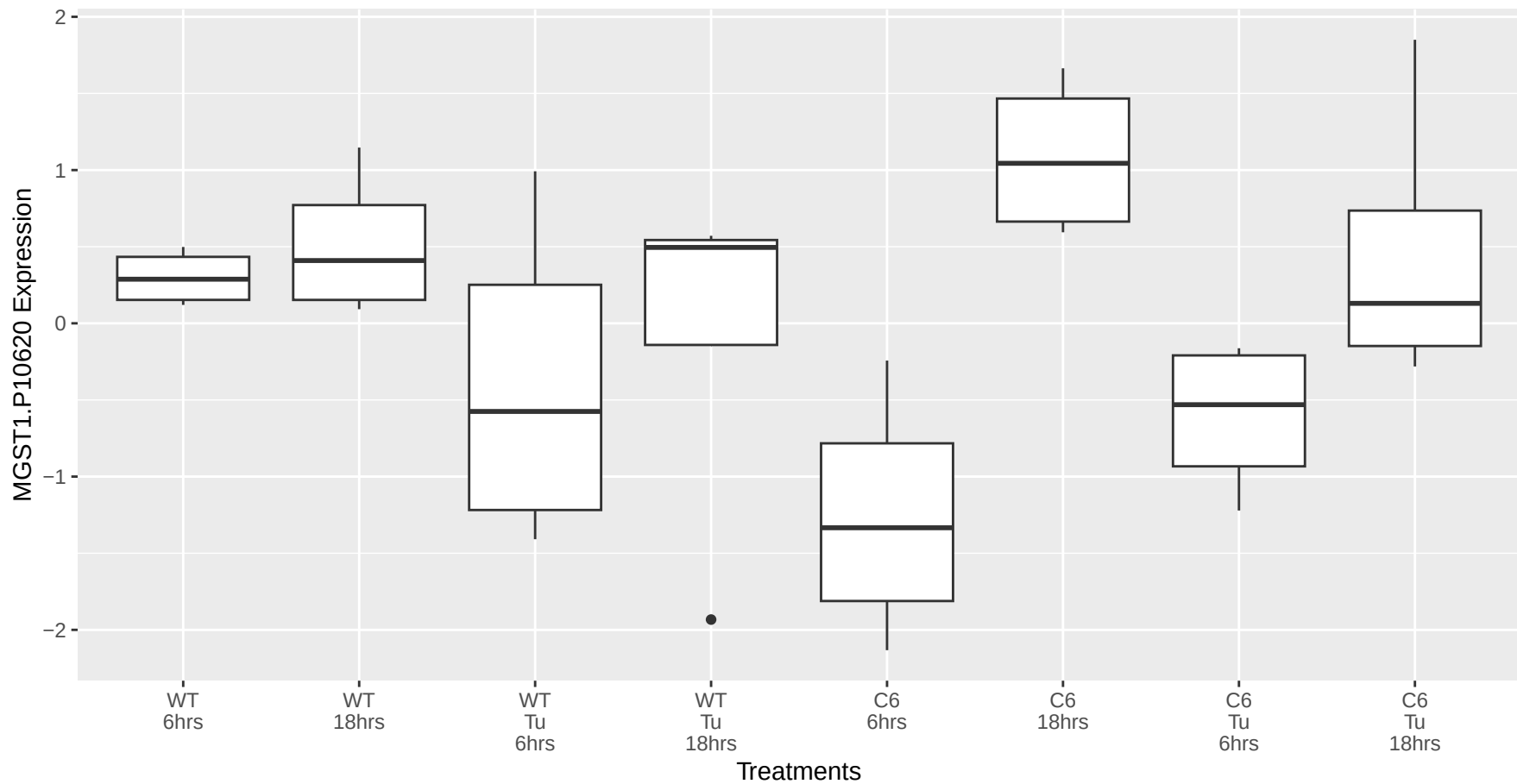
MGST1.P10620 occurs in the yellow module
