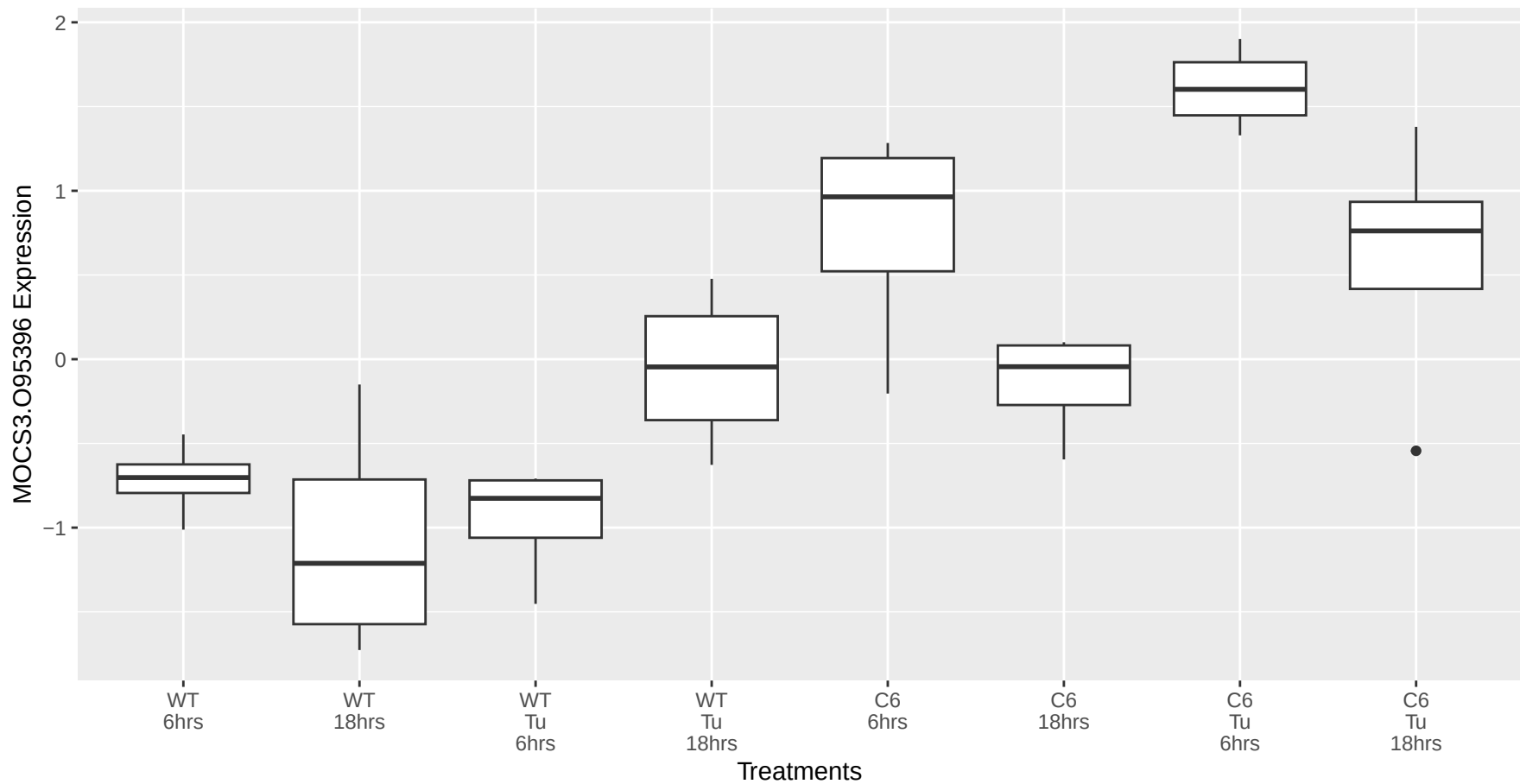
MOCS3.O95396 occurs in the magenta module
