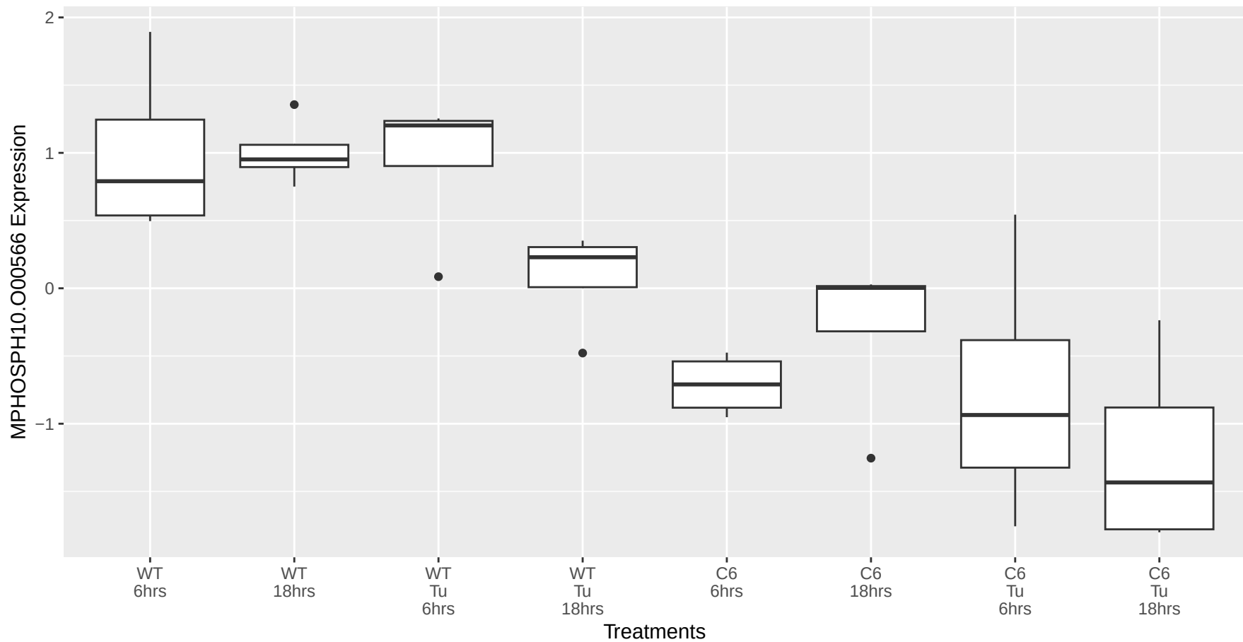
MPHOSPH10.O00566 occurs in the magenta module
