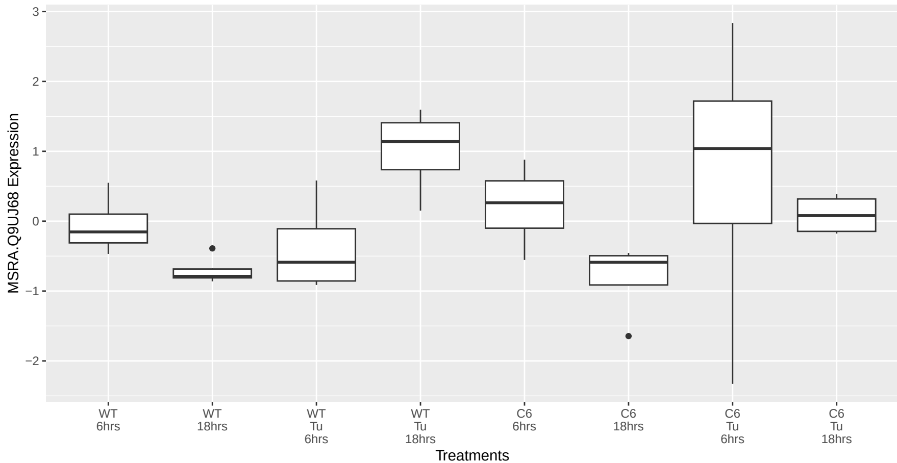
MSRA.Q9UJ68 occurs in the grey module
