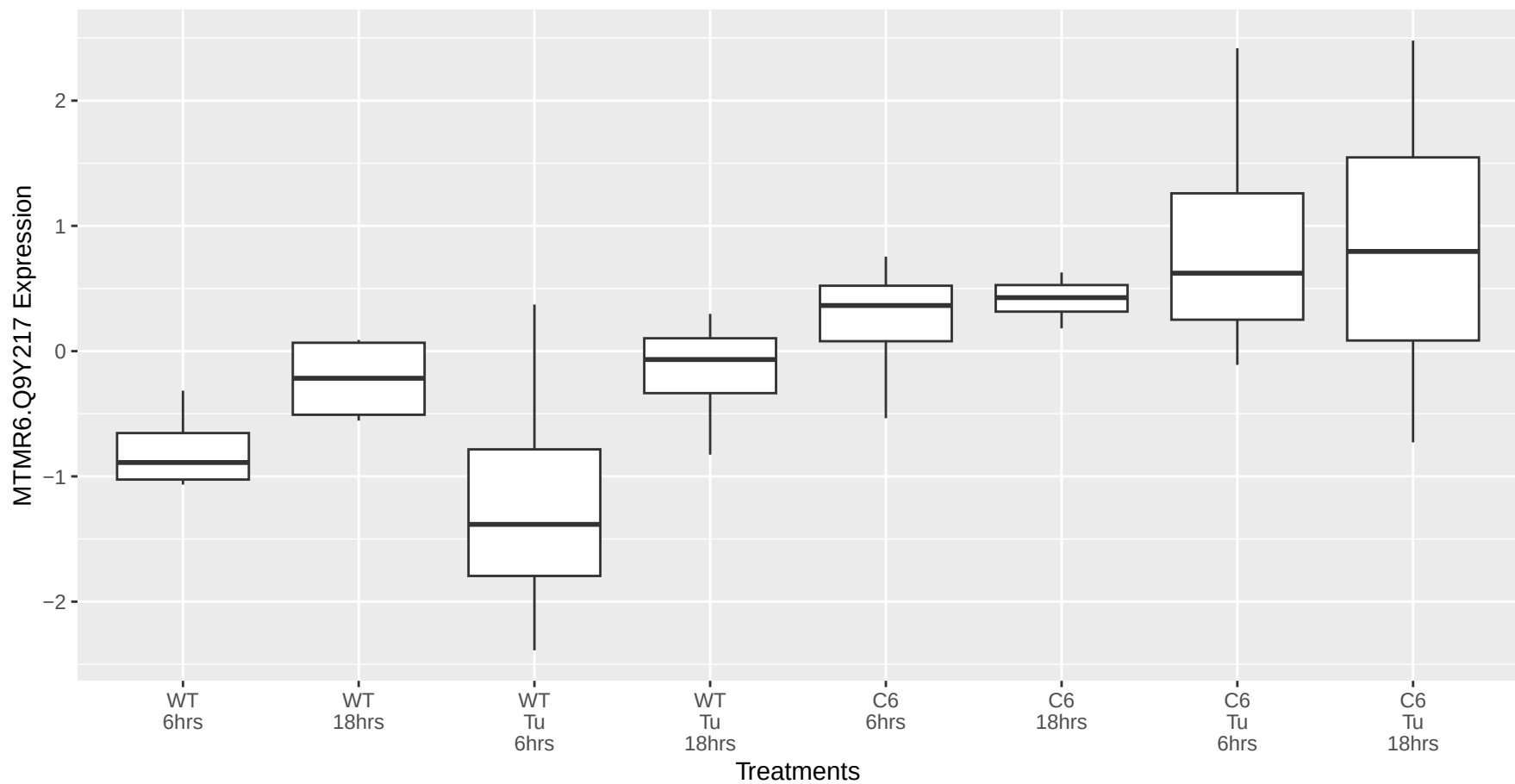
MTMR6.Q9Y217 occurs in the red module
