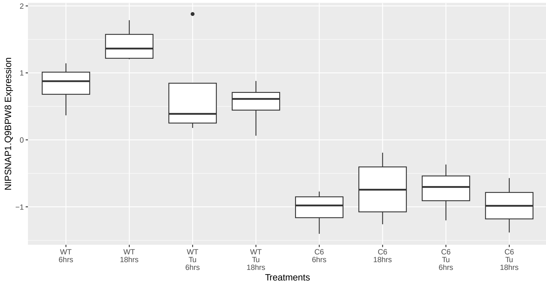
NIPSNAP1.Q9BPW8 occurs in the brown module
