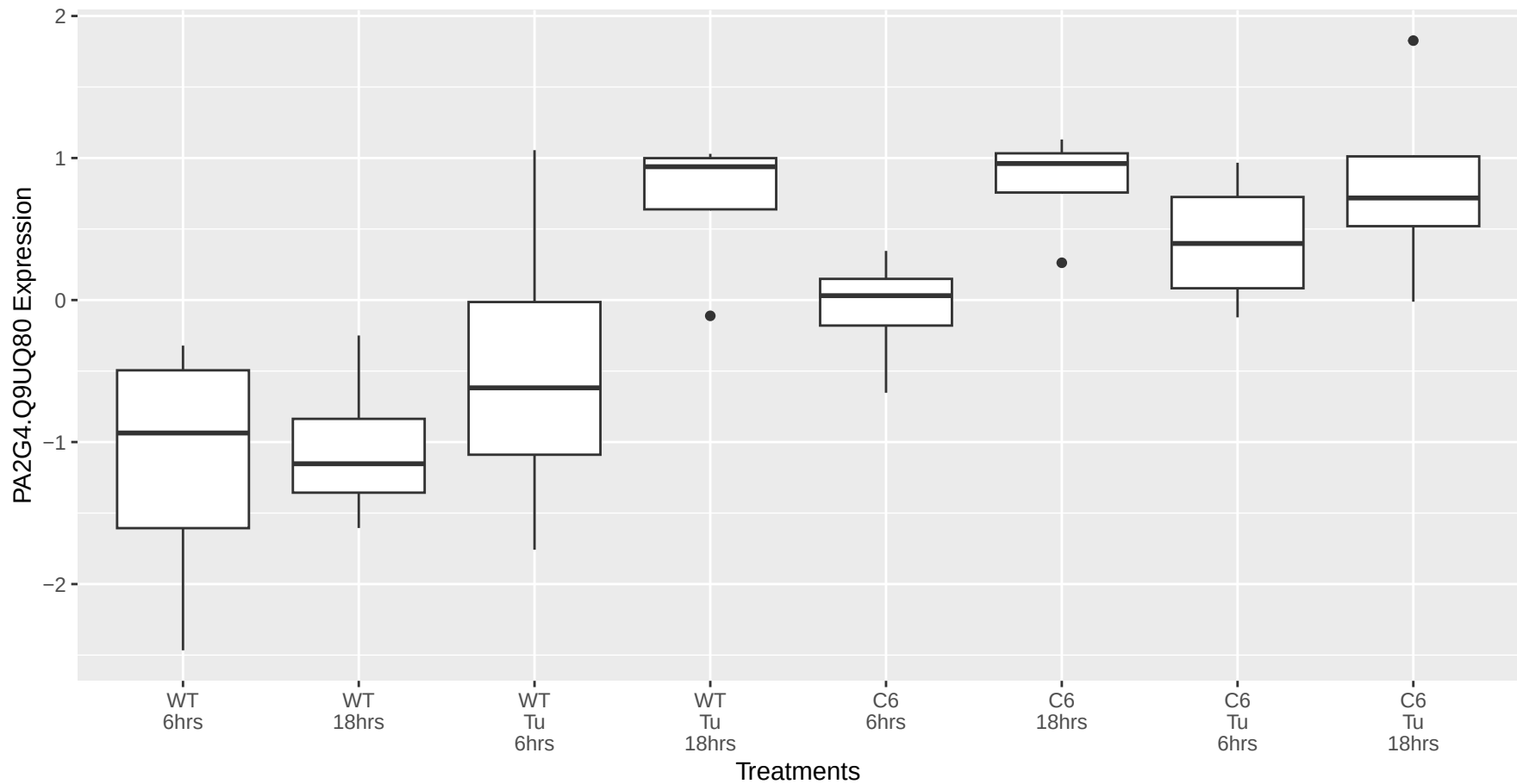
PA2G4.Q9UQ80 occurs in the black module
