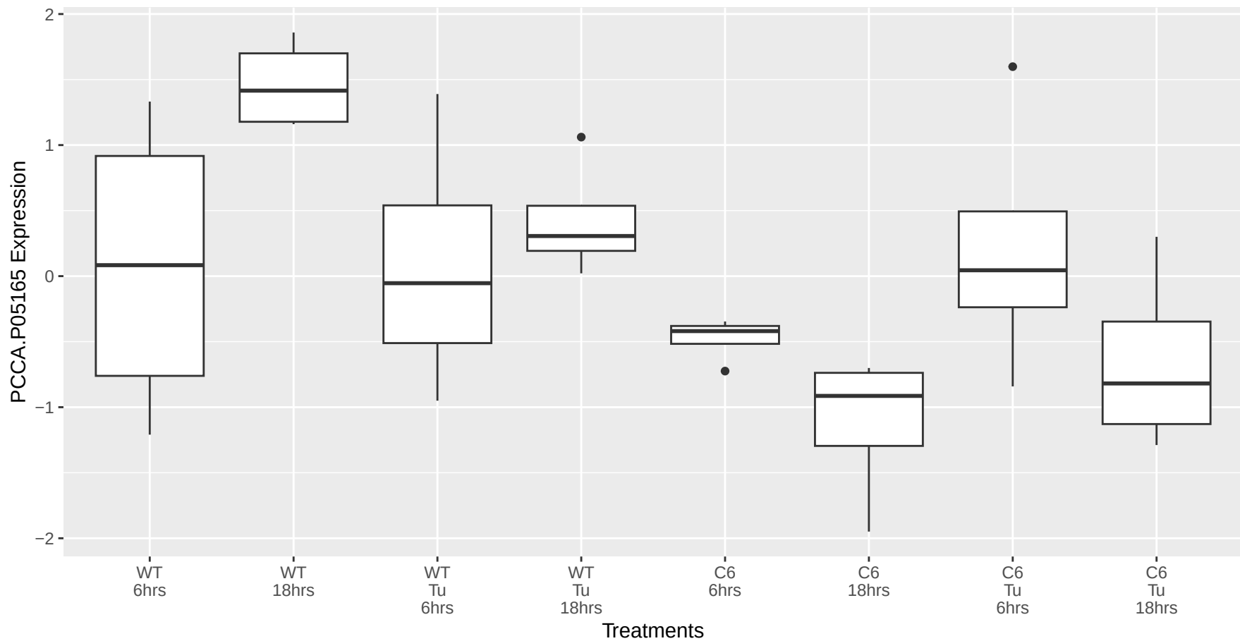
PCCA.P05165 occurs in the brown module
