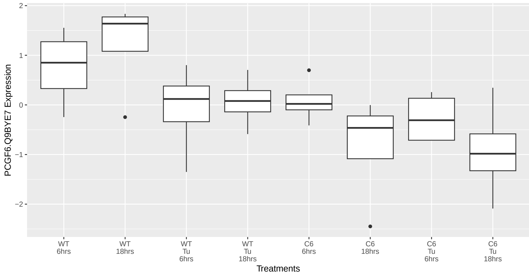
PCGF6.Q9BYE7 occurs in the black module
