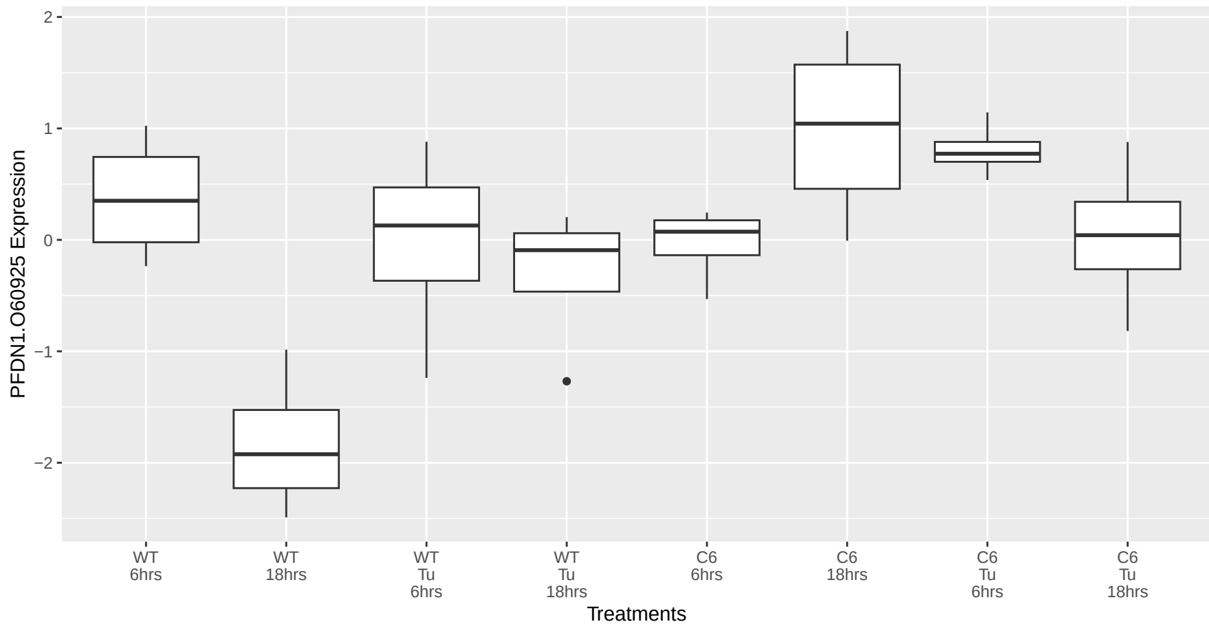
PFDN1.O60925 occurs in the brown module
