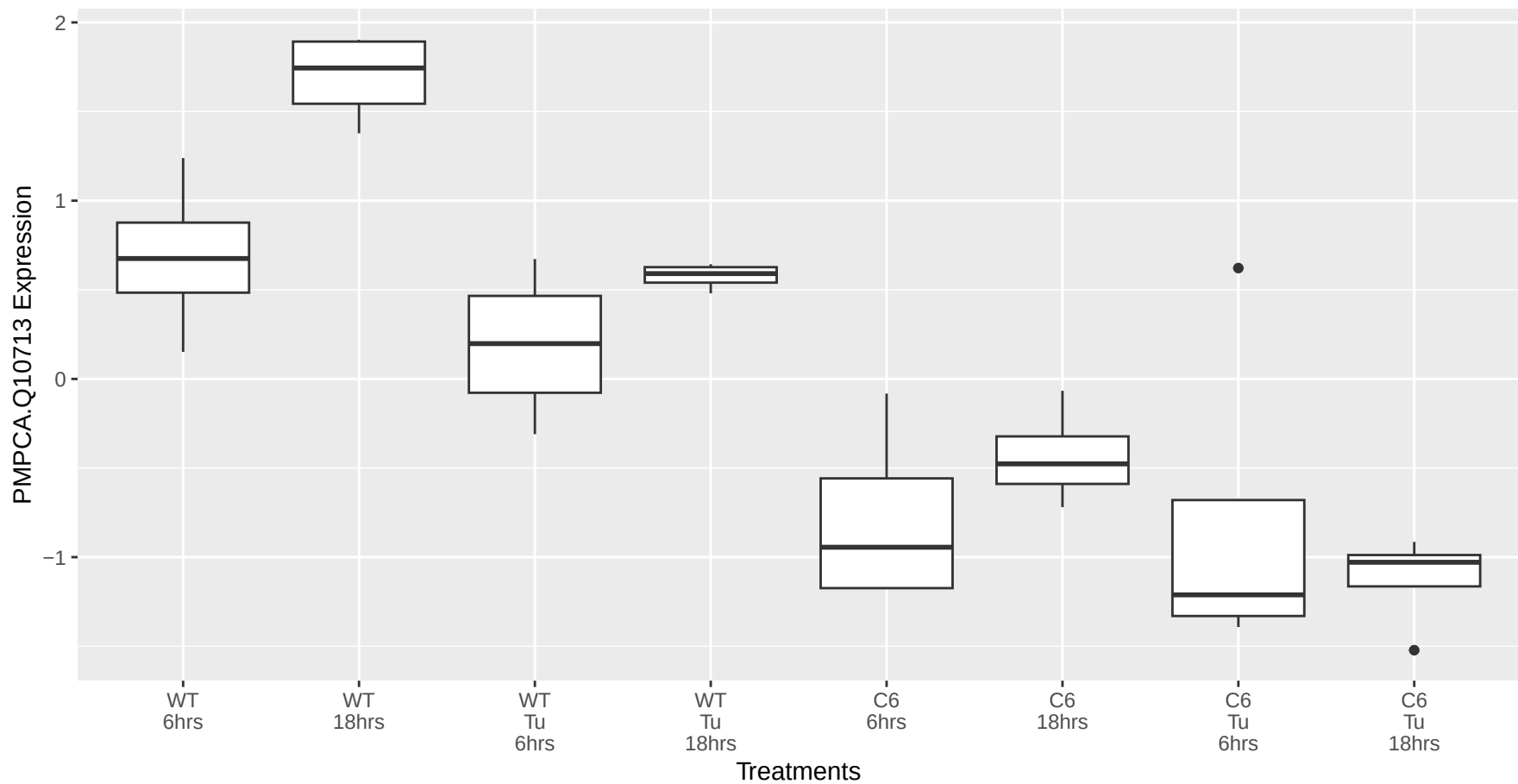
PMPCA.Q10713 occurs in the brown module
