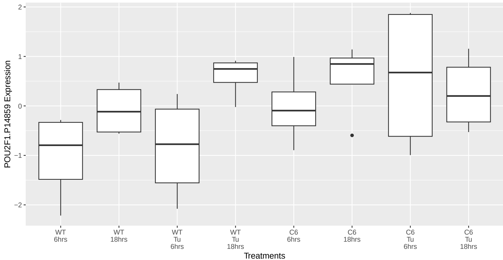
POU2F1.P14859 occurs in the black module
