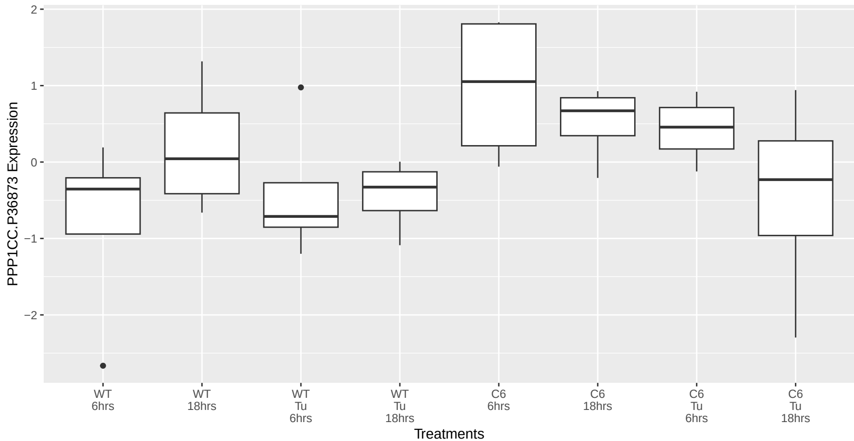
PPP1CC.P36873 occurs in the black module
