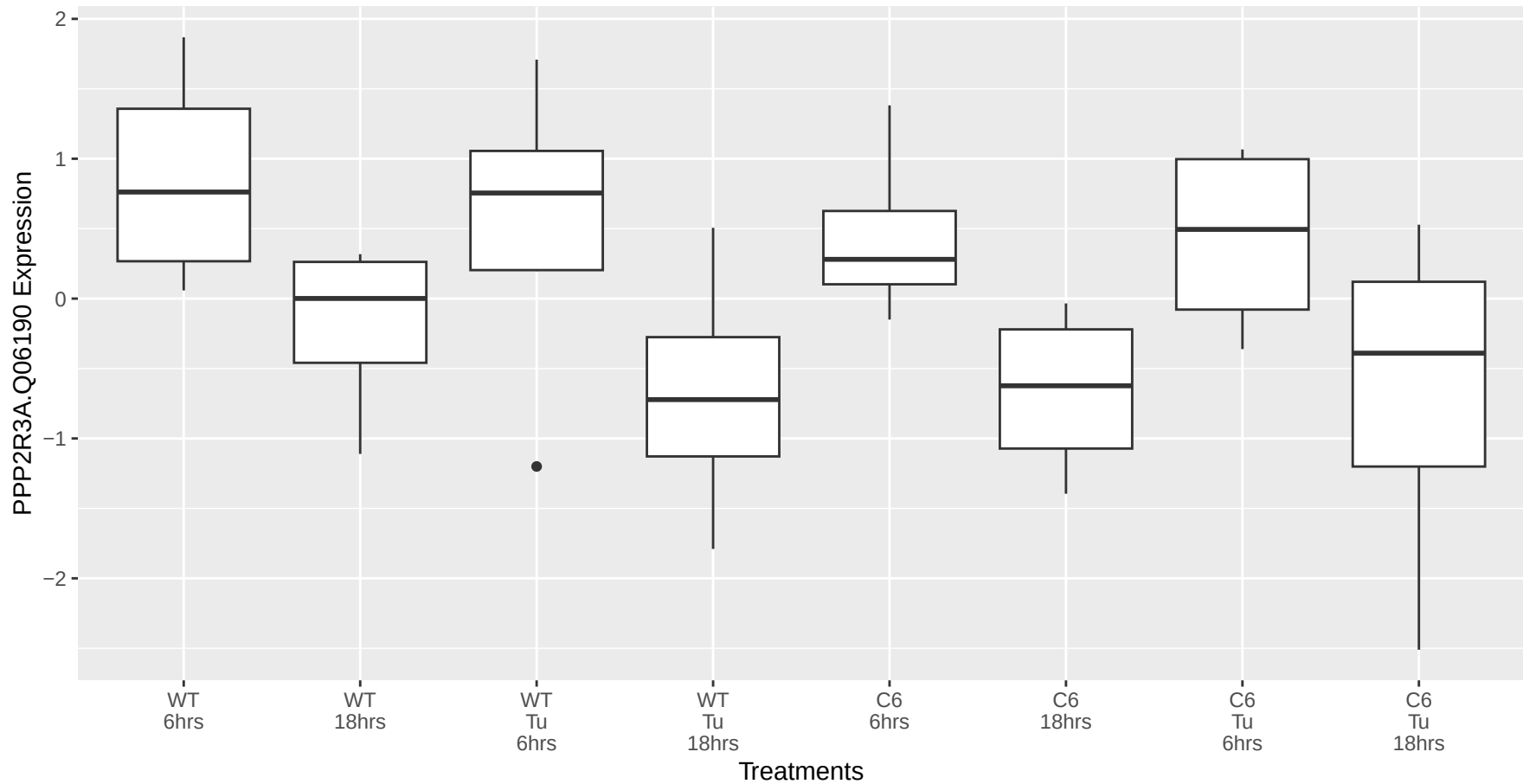
PPP2R3A.Q06190 occurs in the yellow module
