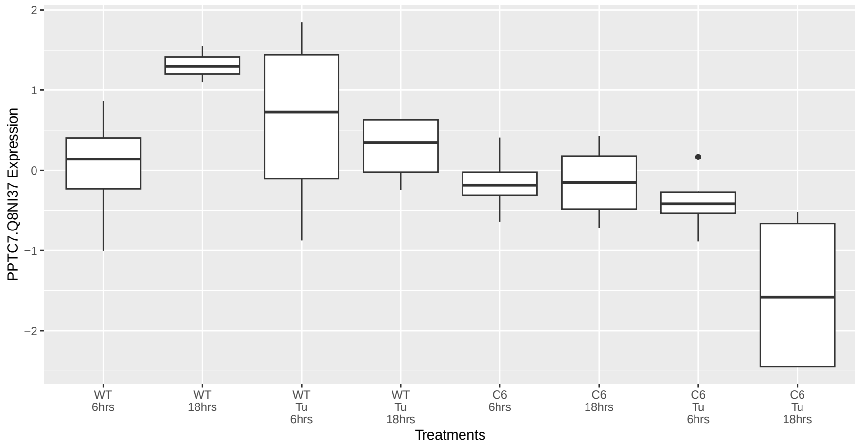
PPTC7.Q8NI37 occurs in the blue module
