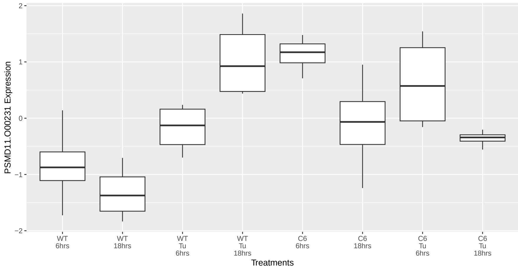
PSMD11.O00231 occurs in the brown module
