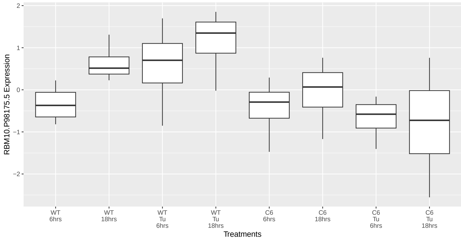
RBM10.P98175.5 occurs in the red module
