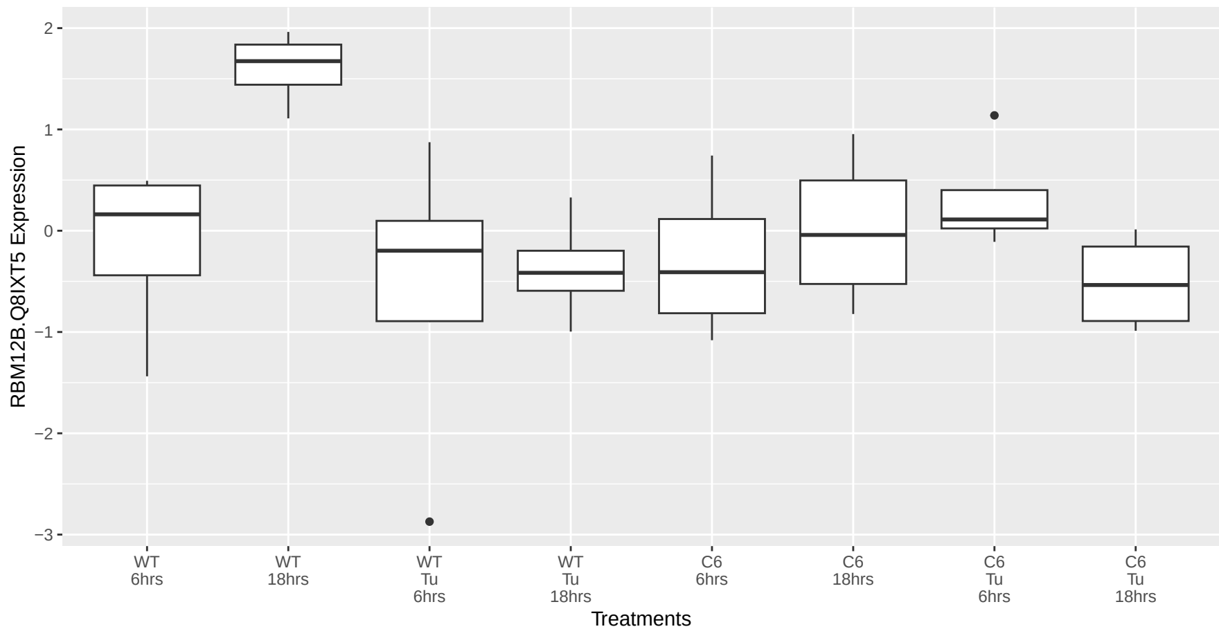
RBM12B.Q8IXT5 occurs in the purple module
