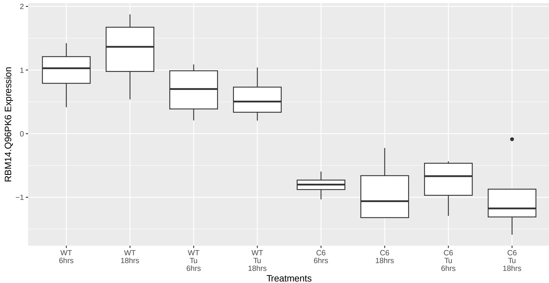
RBM14.Q96PK6 occurs in the magenta module
