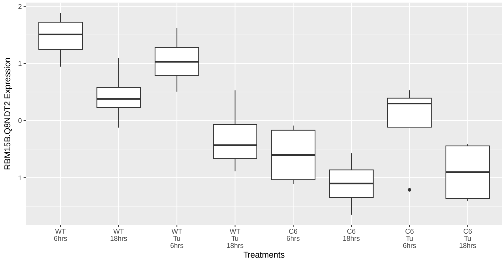
RBM15B.Q8NDT2 occurs in the blue module
