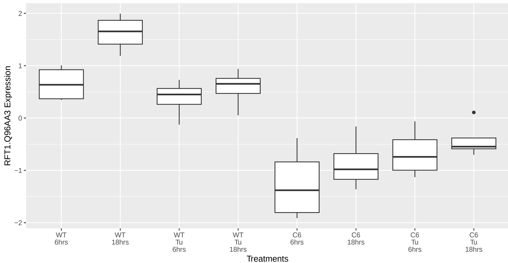
RFT1.Q96AA3 occurs in the brown module
