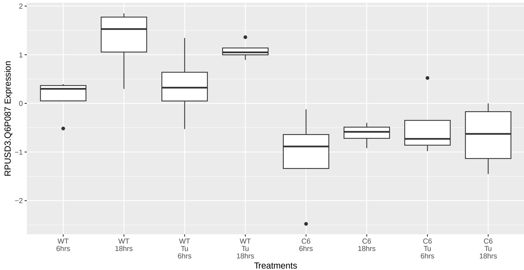
RPUSD3.Q6P087 occurs in the magenta module
