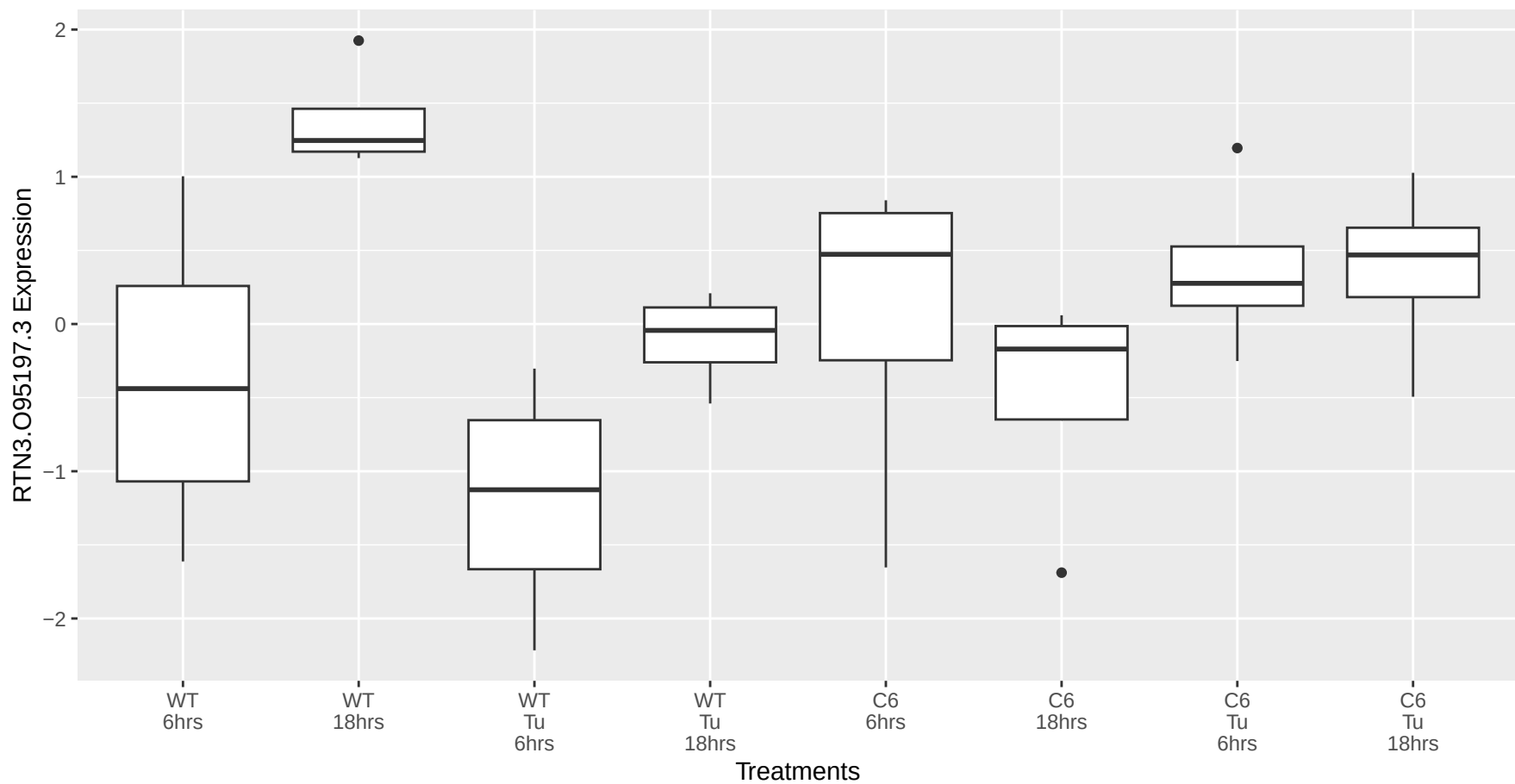
RTN3.O95197.3 occurs in the purple module
