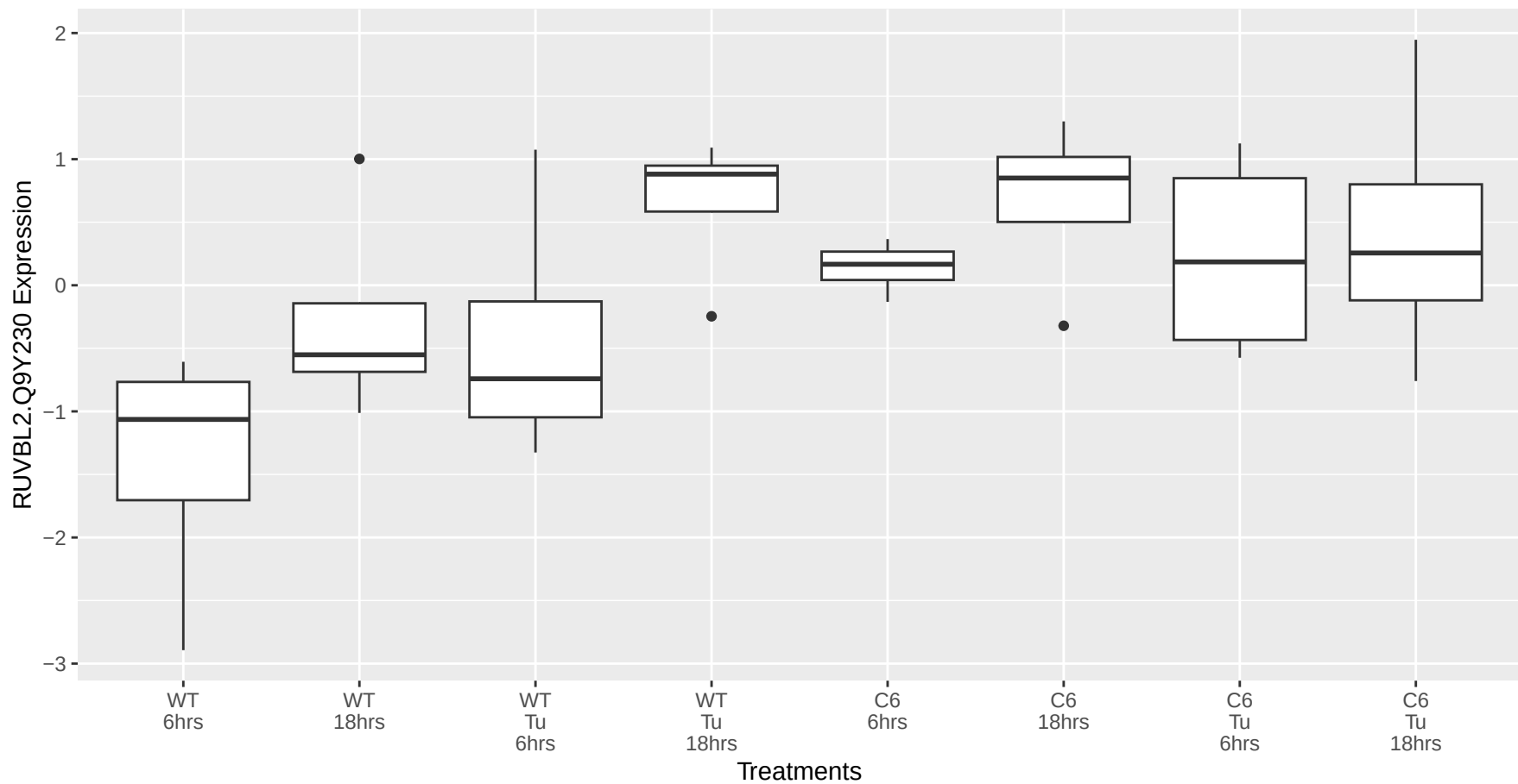
RUVBL2.Q9Y230 occurs in the black module
