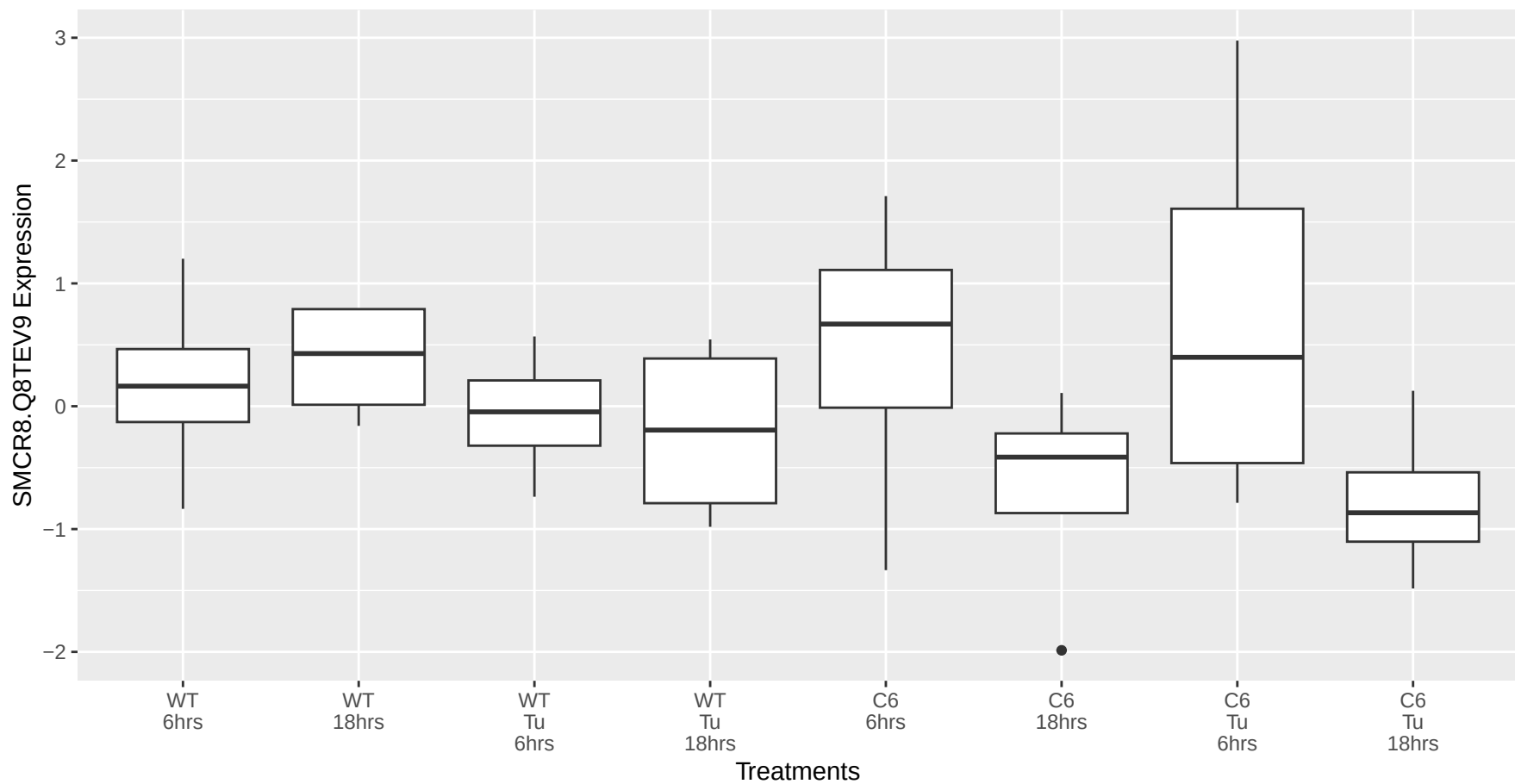
SMCR8.Q8TEV9 occurs in the black module
