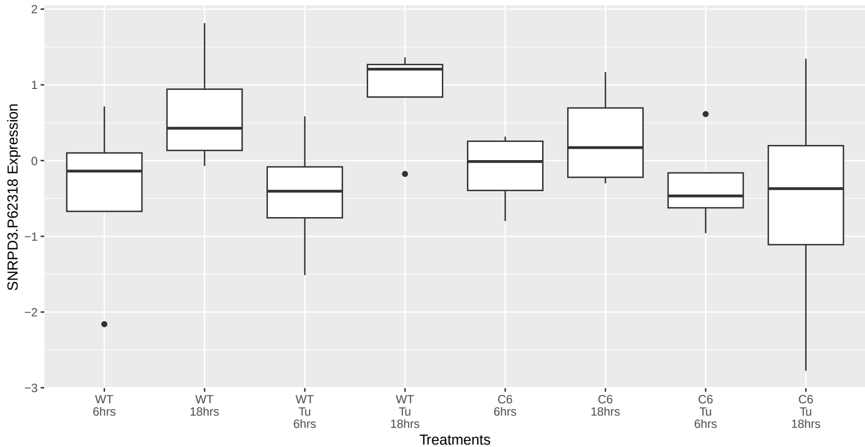
SNRPD3.P62318 occurs in the yellow module
