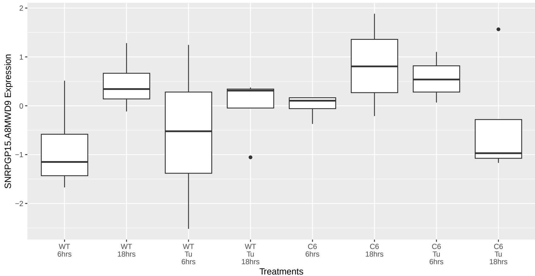
SNRPGP15.A8MWD9 occurs in the yellow module
