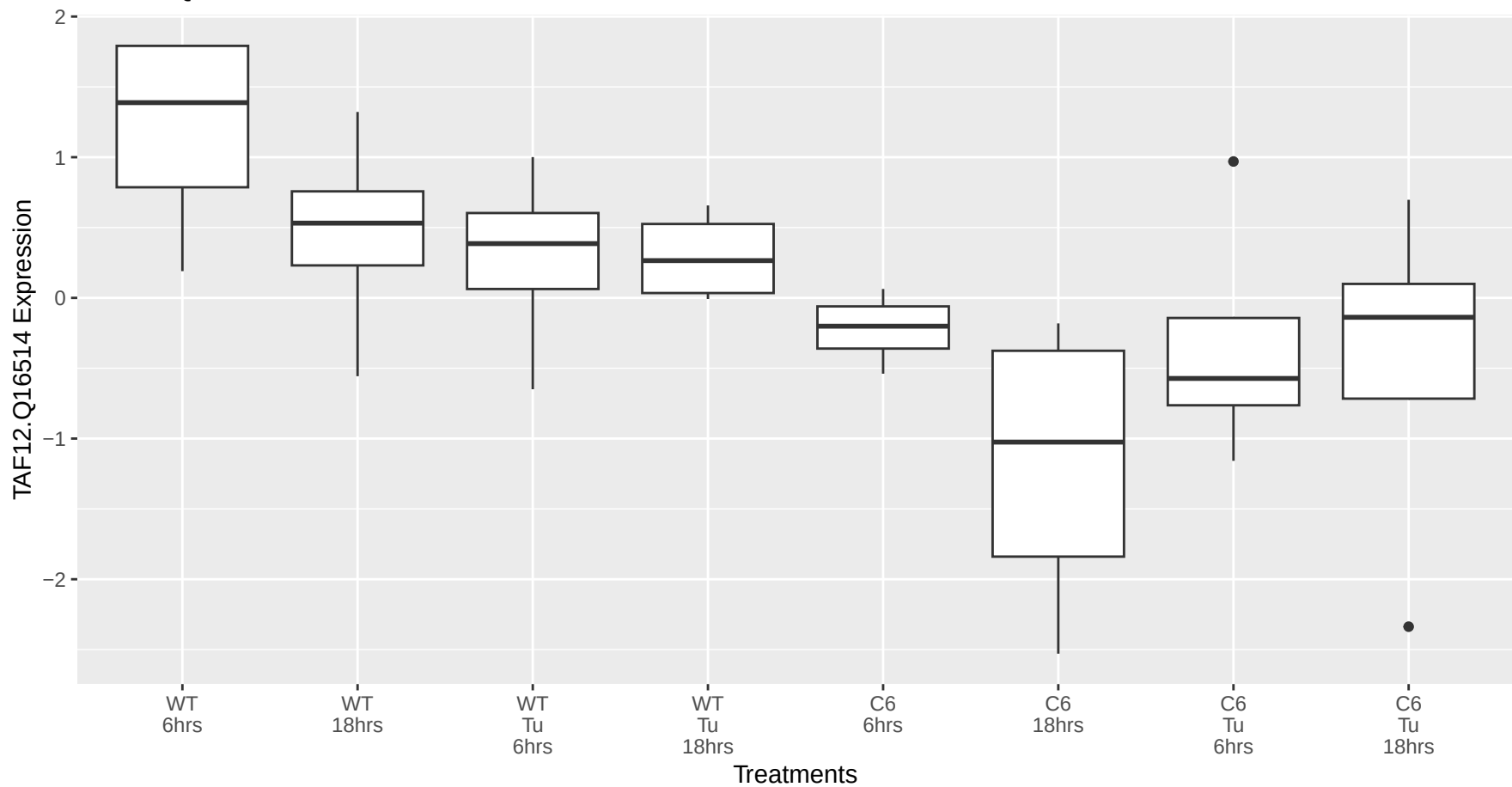
TAF12.Q16514 occurs in the black module
