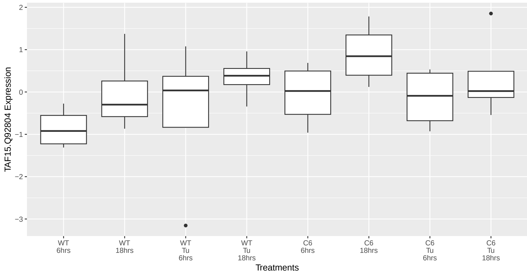
TAF15.Q92804 occurs in the yellow module
