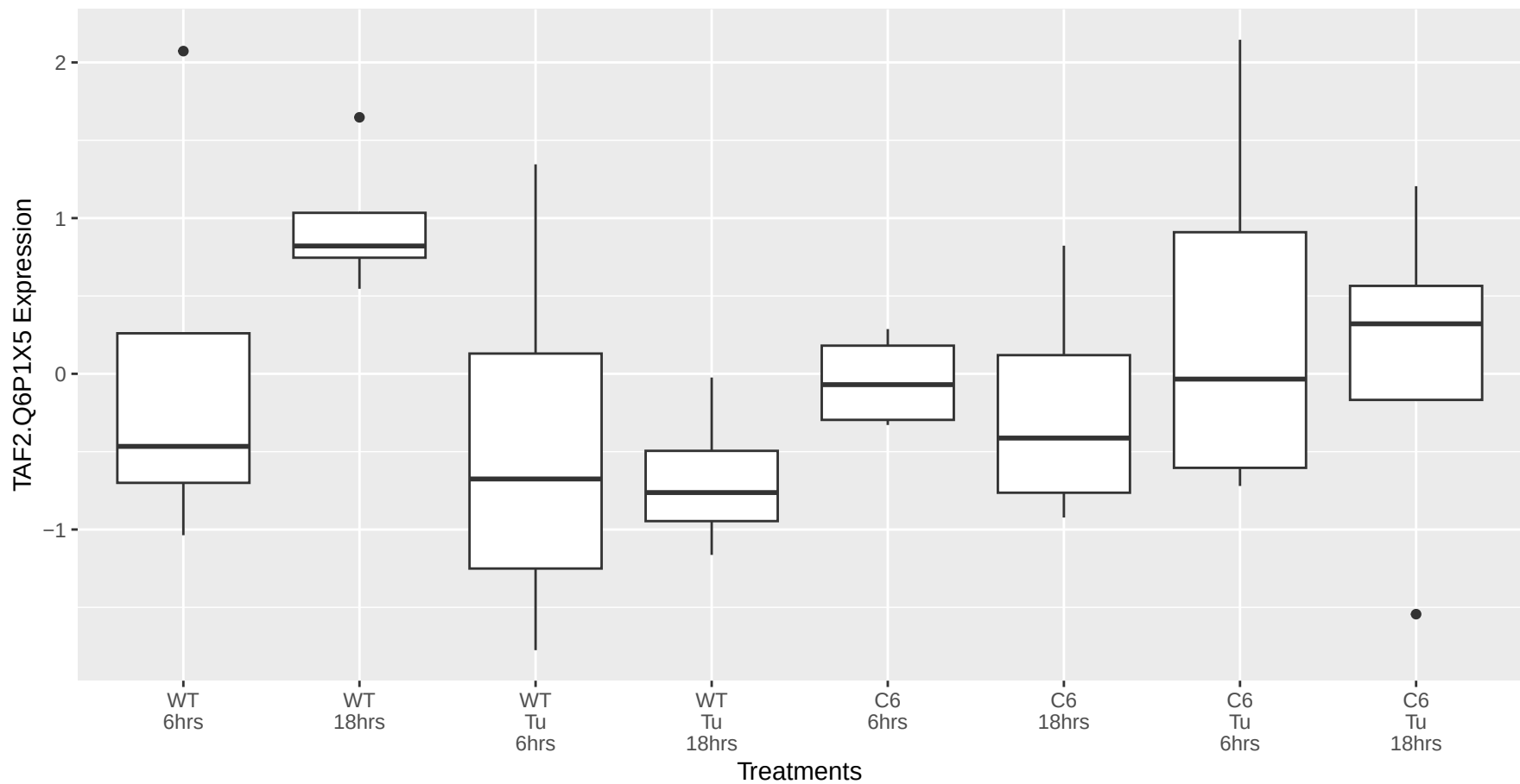
TAF2.Q6P1X5 occurs in the black module
