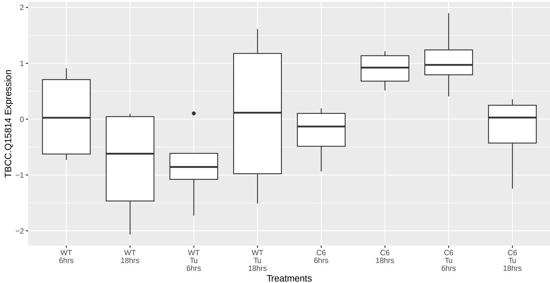
TBCC.Q15814 occurs in the blue module
