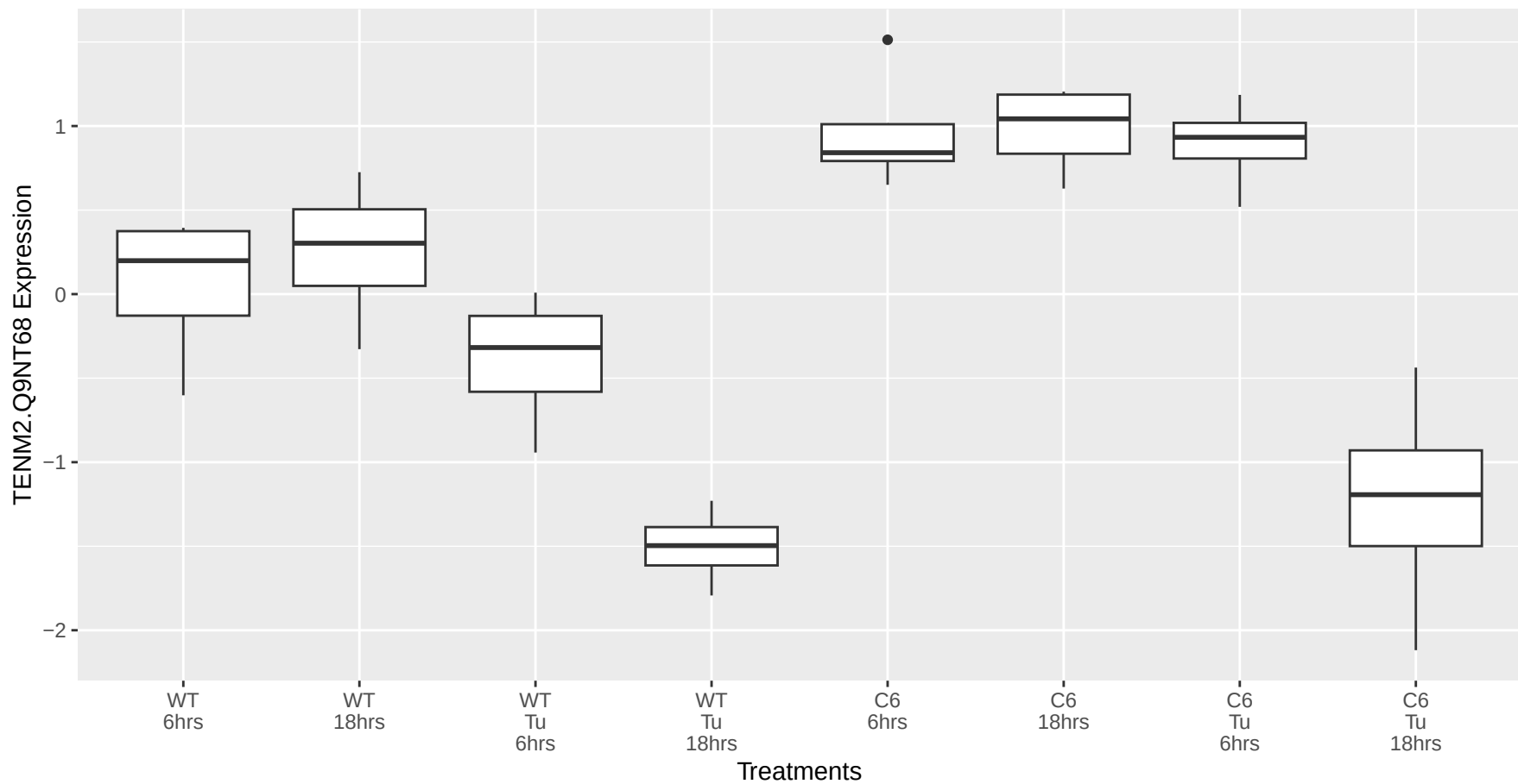
TENM2.Q9NT68 occurs in the cyan module
