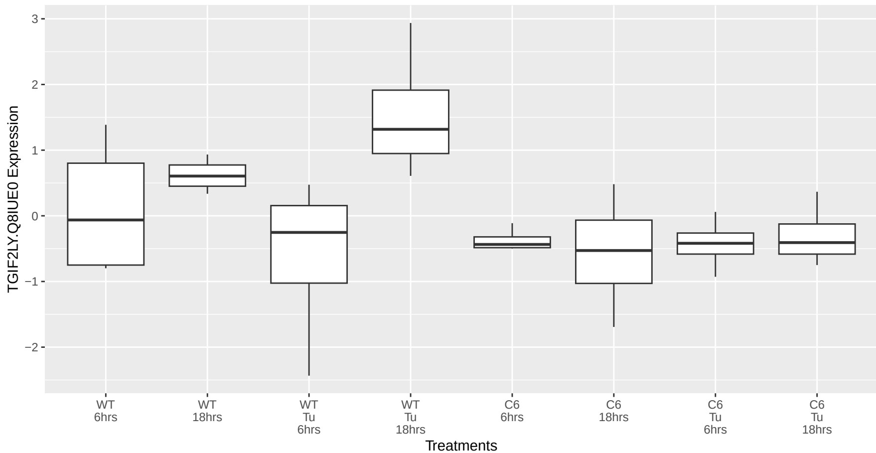
TGIF2LY.Q8IUOE0 occurs in the magenta module
