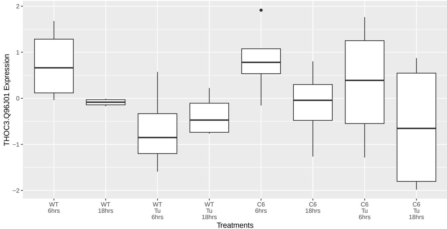
THOC3.Q96J01 occurs in the grey module
