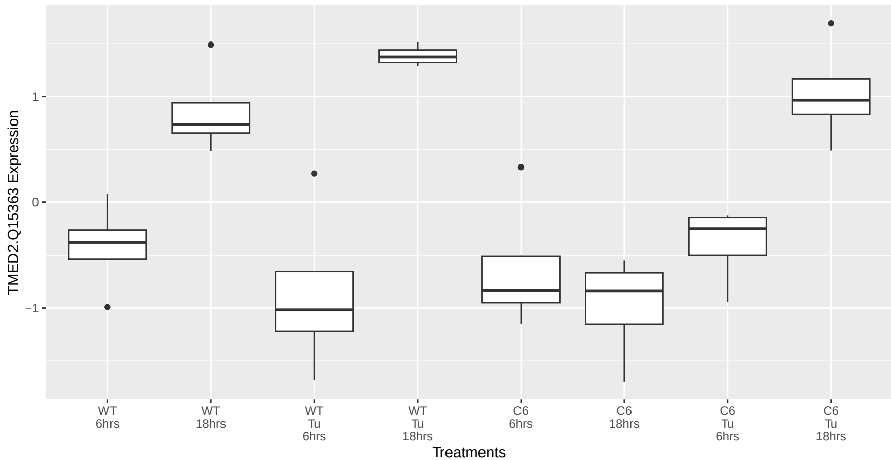
TMED2.Q15363 occurs in the cyan module
