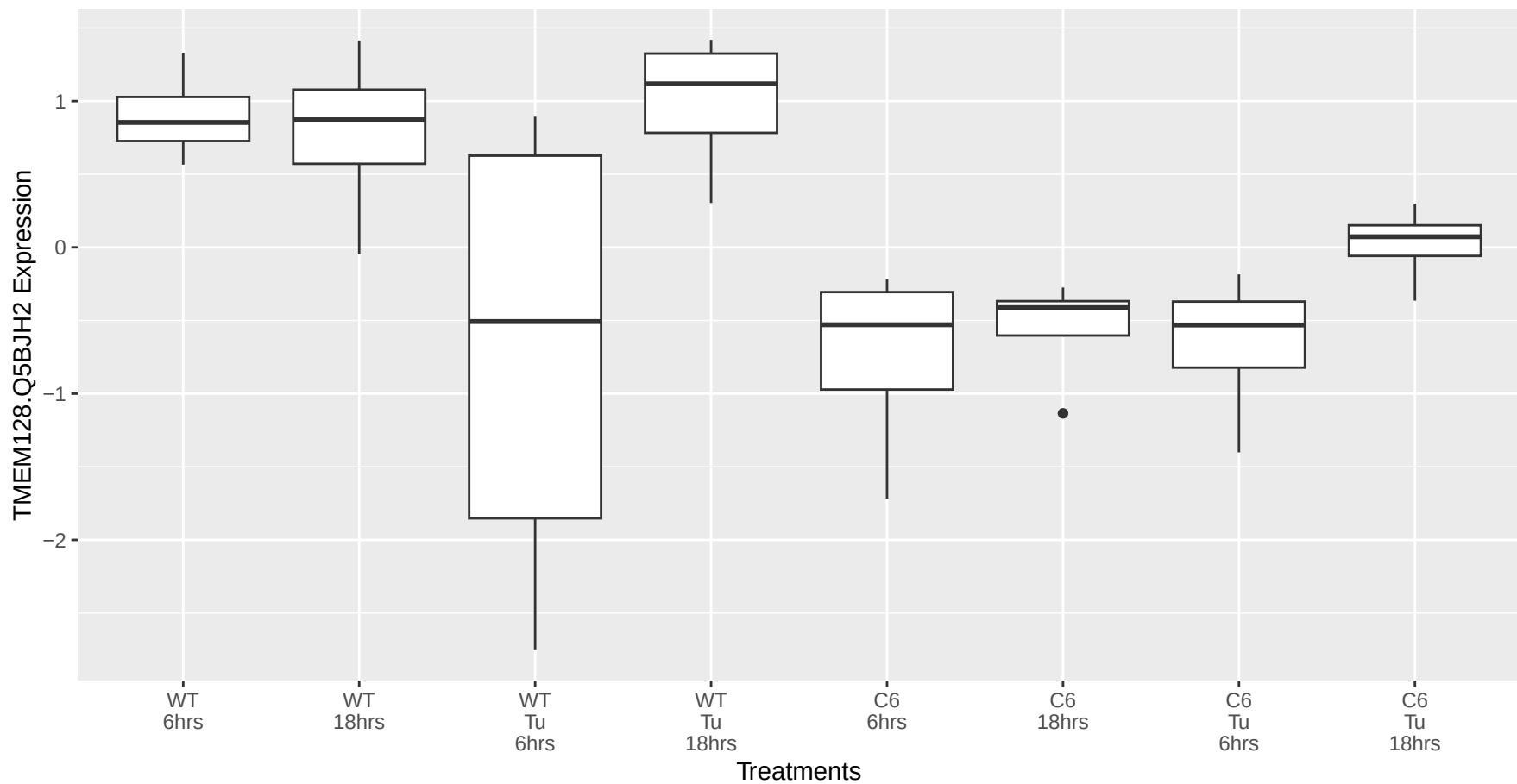
TMEM128.Q5BJH2 occurs in the magenta module
