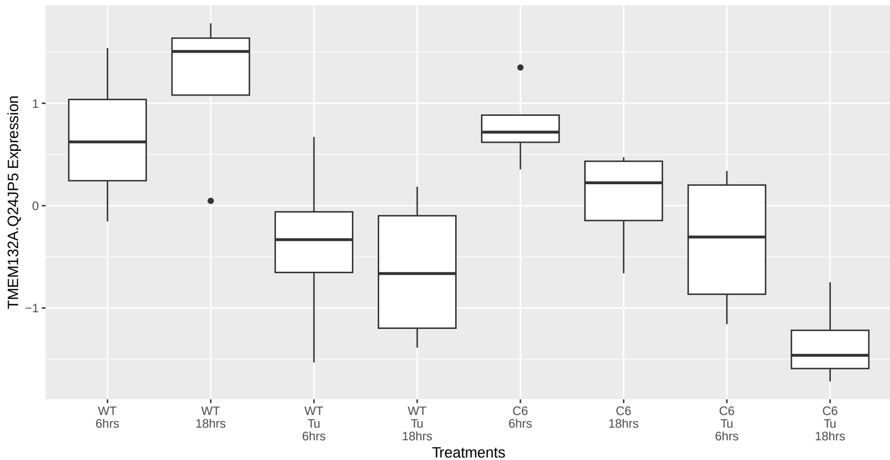
TMEM132A.Q24JP5 occurs in the blue module
