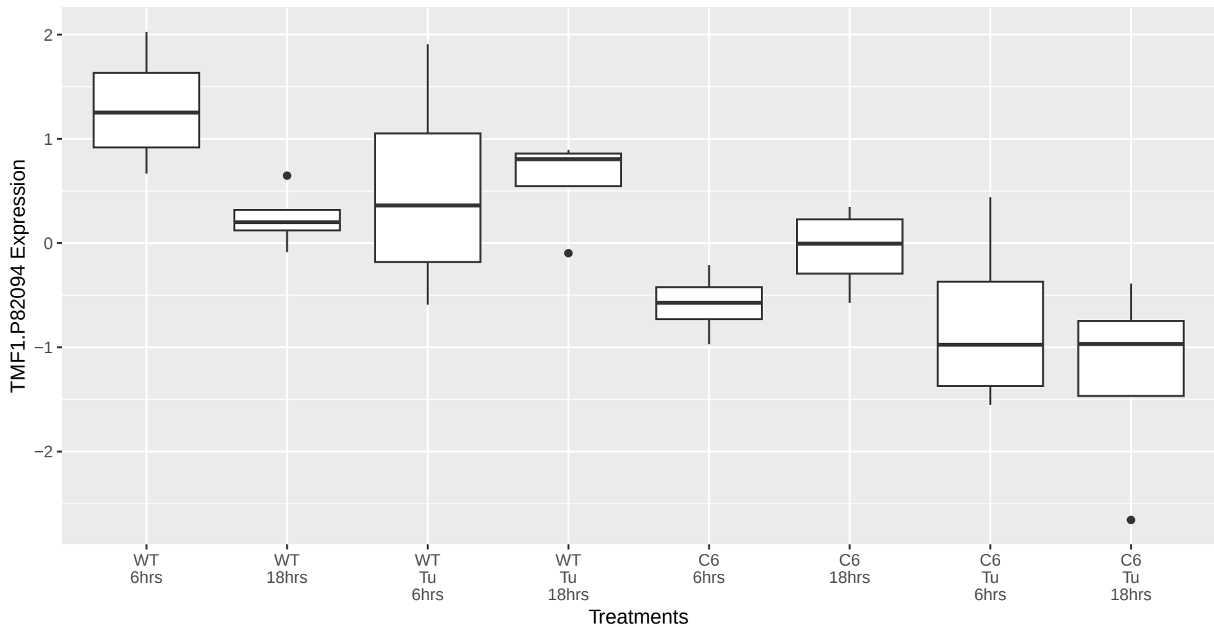
TMF1.P82094 occurs in the magenta module
