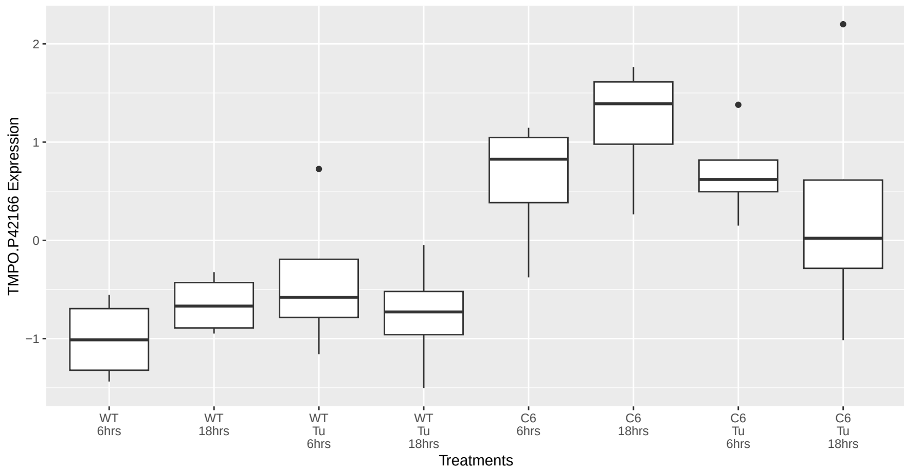
TMPO.P42166 occurs in the greenyellow module
