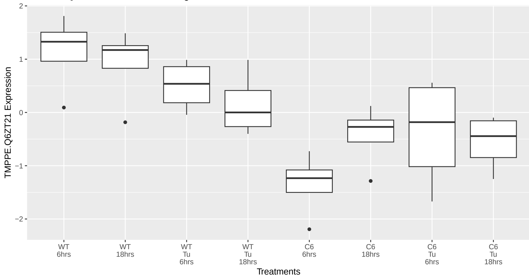
TMPPE.Q6ZT21 occurs in the magenta module
