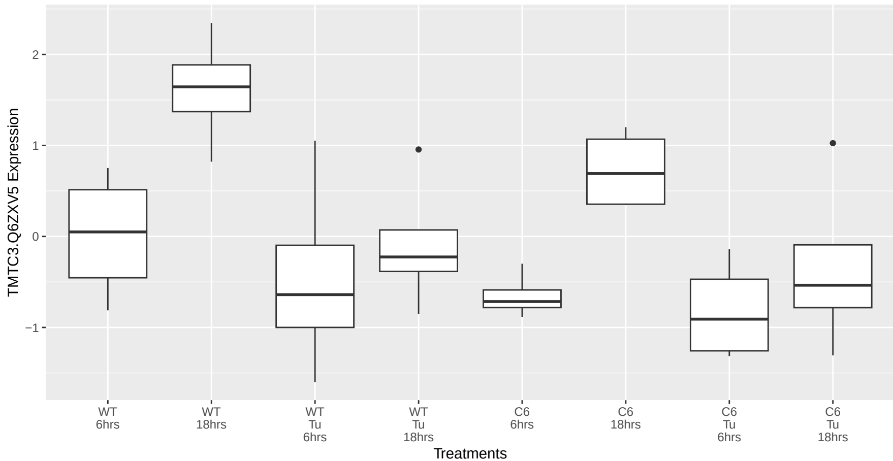
TMTC3.Q6ZXV5 occurs in the brown module
